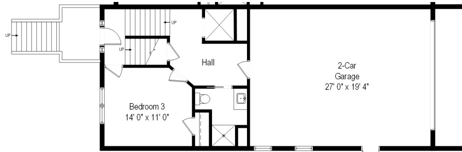
FIRST LEVEL
