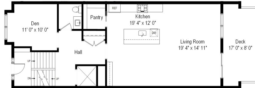
SECOND LEVEL
