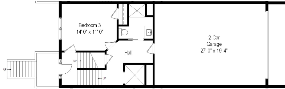
FIRST LEVEL
